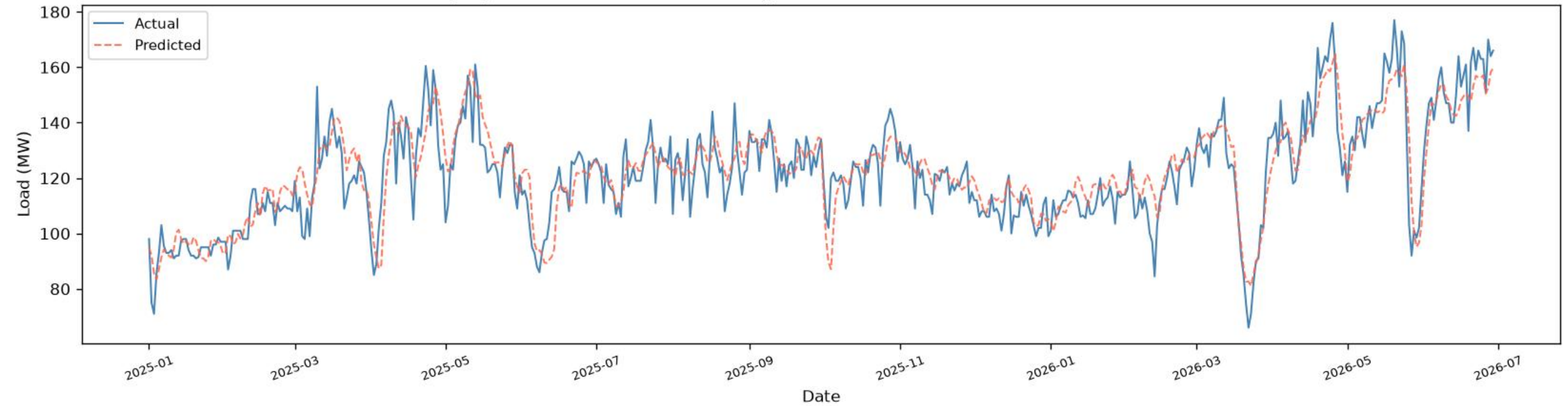
Mirpur | BiLSTM - TEST ( \geq 2025 ), one-day-ahead ( R^2=0.7782 , RMSE=8.86 , MAE=6.80 , n=528 )
