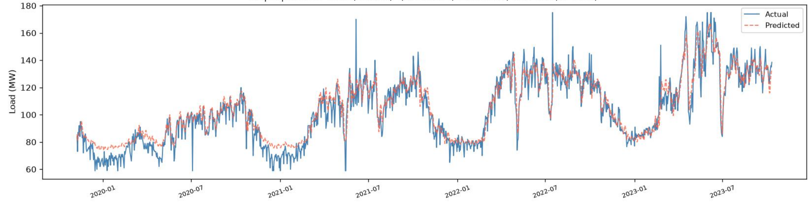
Mirpur | BiLSTM - TRAIN (fit block) ( R^2=0.8973 , RMSE=7.84, MAE=5.76, n=1396)
