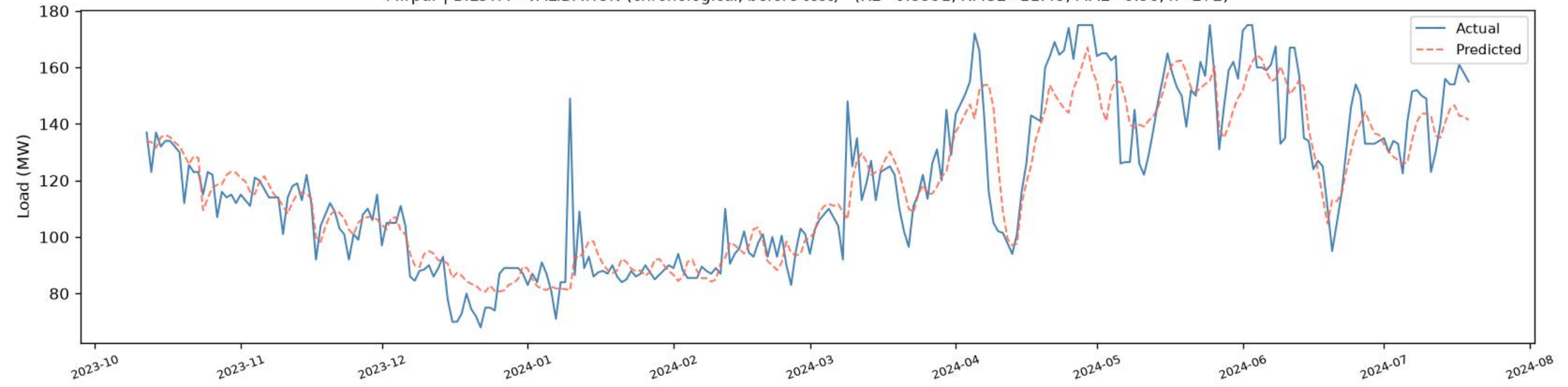
Mirpur | BiLSTM - VALIDATION (chronological, before test) ( R^2=0.8351 , RMSE=11.45, MAE=8.36, n=272 )
