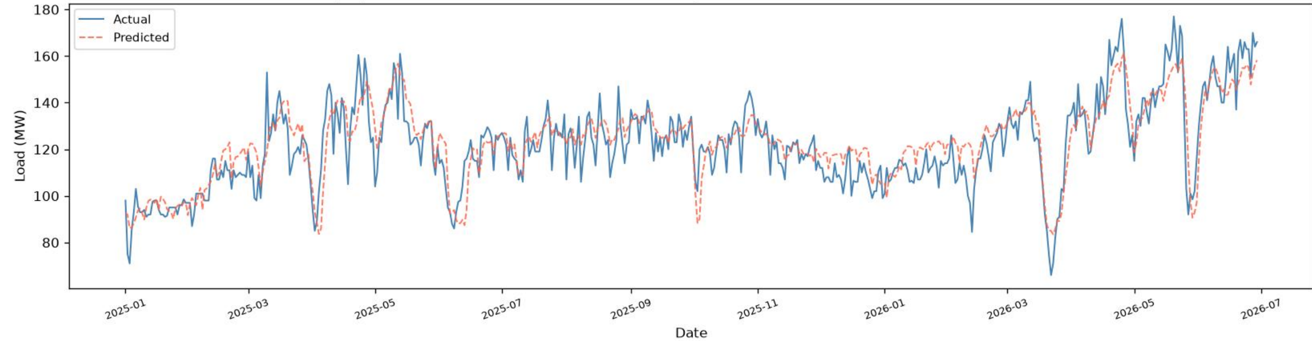
Mirpur | CNN+BiGRU+BiLSTM - TEST ( \geq 2025 ), one-day-ahead ( R^2=0.7482 , RMSE=9.44, MAE=7.23, n=528 )
