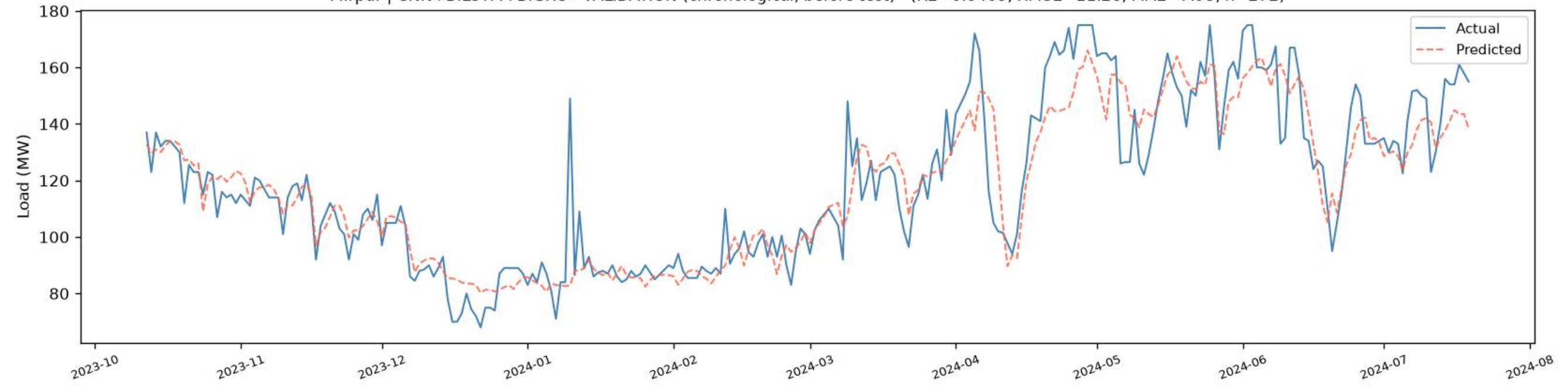
Mirpur | CNN+BiLSTM+BiGRU - VALIDATION (chronological, before test) ( R^2=0.8405 , RMSE=11.26 , MAE=7.95 , n=272 )
