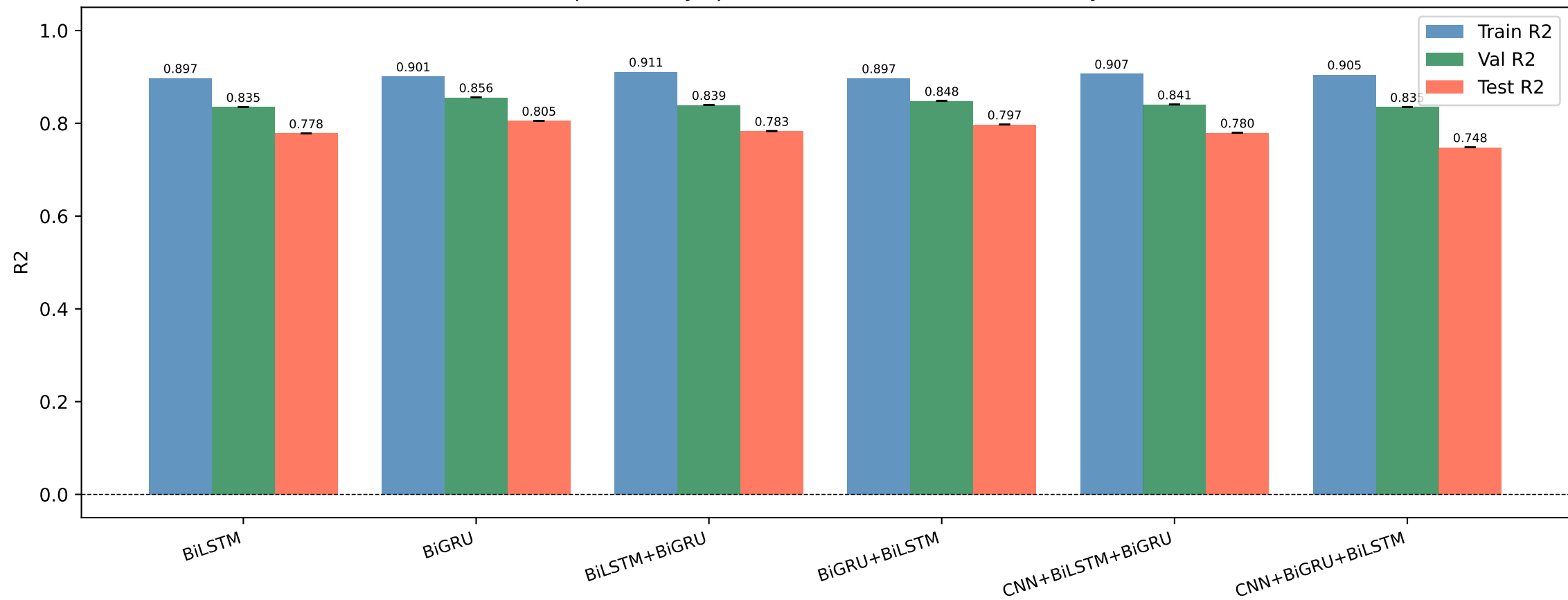
Mirpur - R2 by split (model selection uses VAL only)
