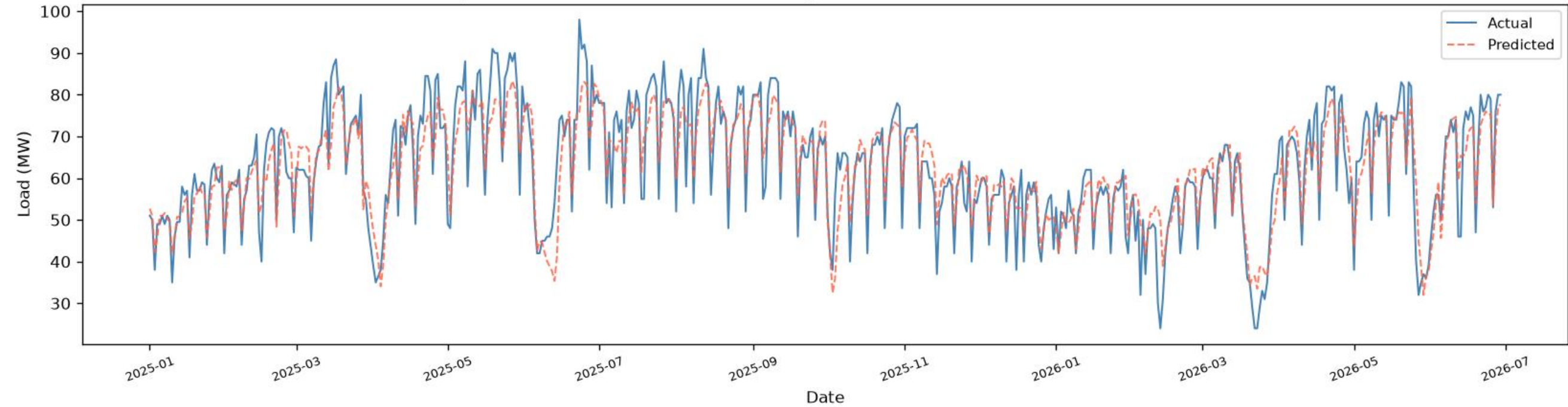
Narinda | BiGRU+BiLSTM - TEST ( \geq 2025 ), one-day-ahead ( R^2=0.8048 , RMSE=6.30 , MAE=4.87 , n=536 )
