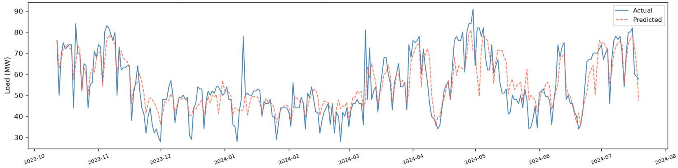
Narinda | BiGRU+BiLSTM - VALIDATION (chronological, before test) ( R^2=0.6756 , RMSE=8.23 , MAE=6.04 , n=272 )
