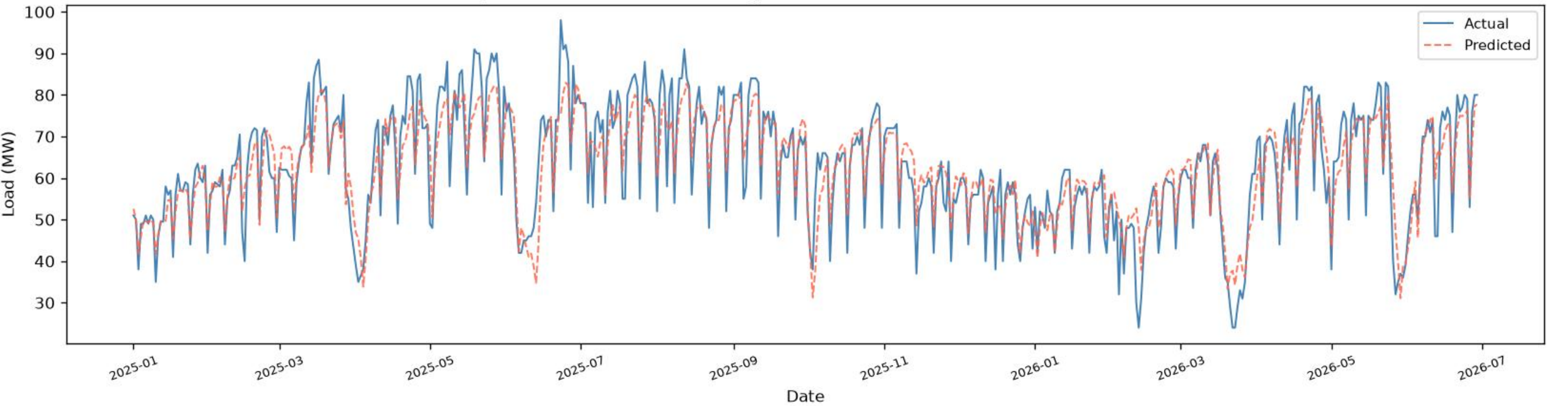
Narinda | BiGRU - TEST ( \geq 2025 ), one-day-ahead ( R^2=0.8104 , RMSE=6.21 , MAE=4.73 , n=536 )
