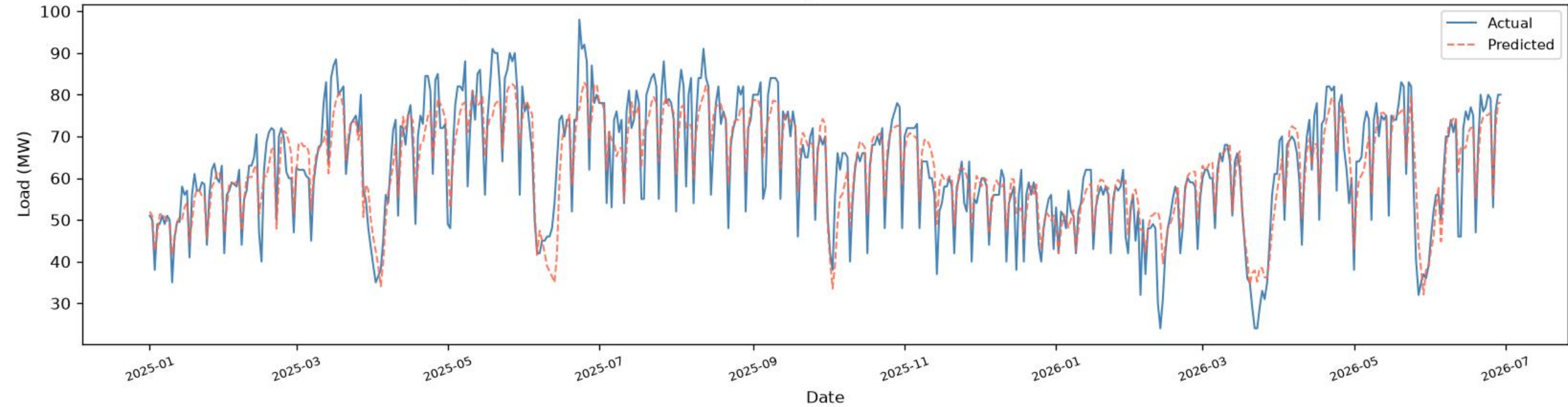
Narinda | BiLSTM+BiGRU - TEST ( \geq 2025 ), one-day-ahead ( R^2=0.8058 , RMSE=6.28 , MAE=4.88 , n=536 )
