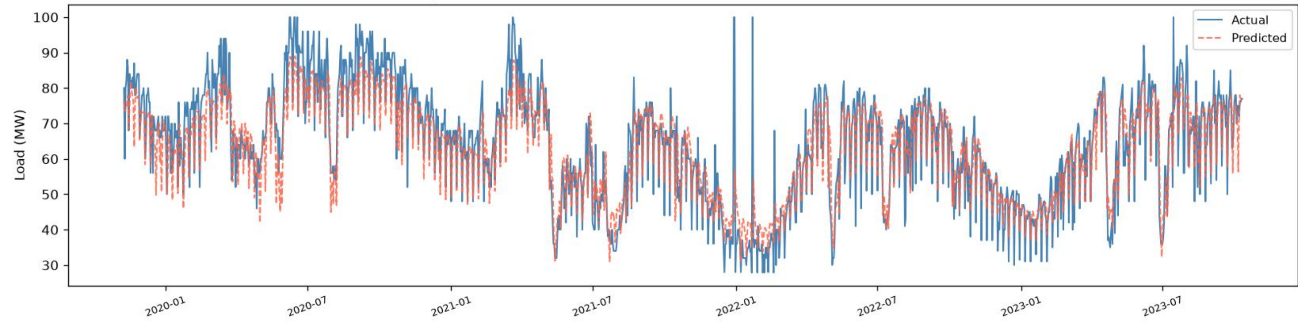
Narinda | BiLSTM+BiGRU - TRAIN (fit block) (R2=0.8149, RMSE=6.97, MAE=5.07, n=1398)
