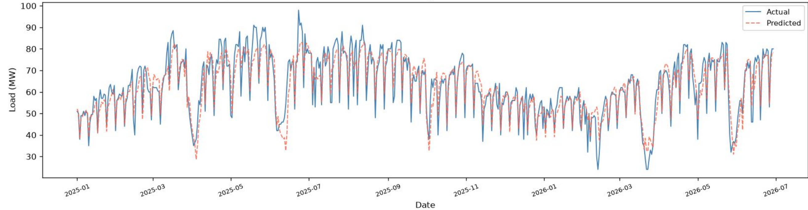
Narinda | CNN+BiGRU+BiLSTM - TEST ( \geq 2025 ), one-day-ahead ( R^2=0.8342 , RMSE=5.80 , MAE=4.39 , n=536 )
