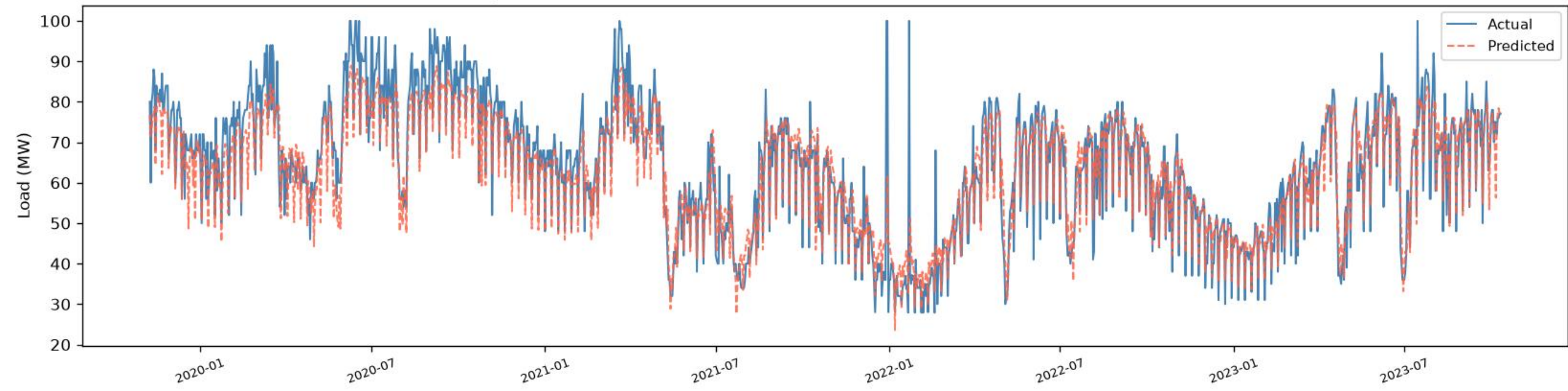
Narinda | CNN+BiGRU+BiLSTM - TRAIN (fit block) (R2=0.8477, RMSE=6.32, MAE=4.50, n=1398)
