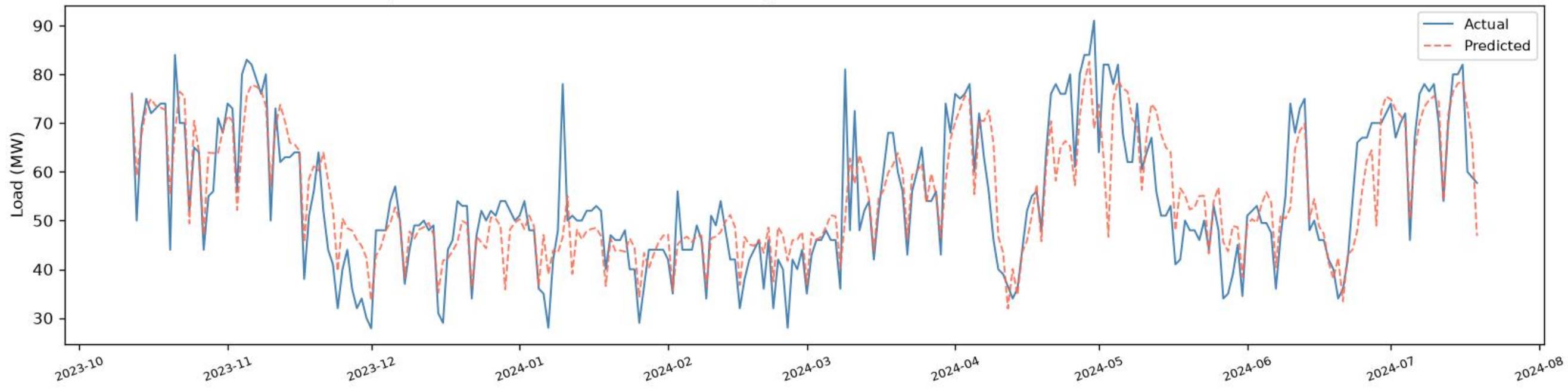
Narinda | CNN+BiGRU+BiLSTM - VALIDATION (chronological, before test) ( R^2=0.7068 , RMSE=7.82 , MAE=5.70 , n=272 )
