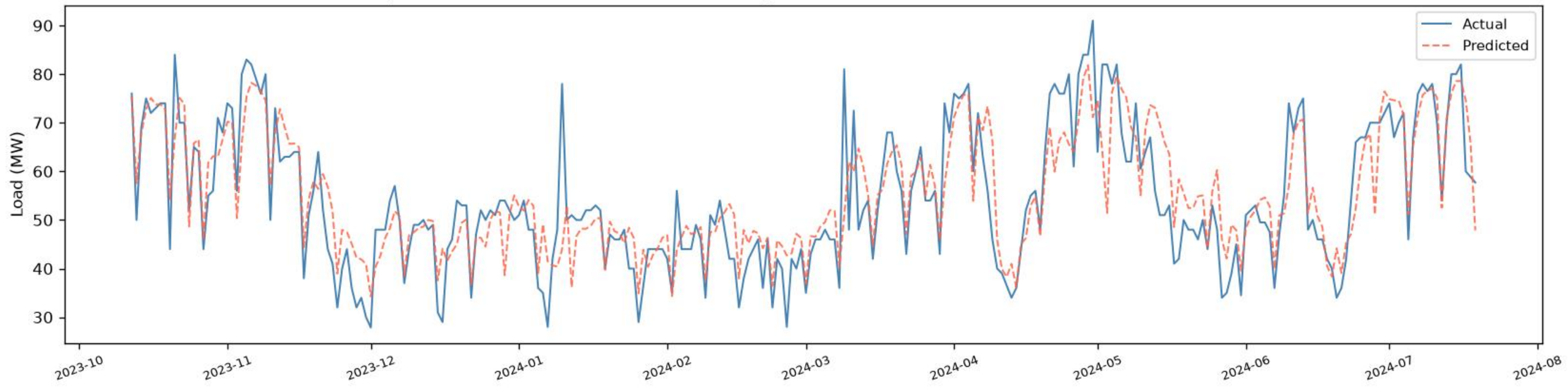
Narinda | CNN+BiLSTM+BiGRU - VALIDATION (chronological, before test) ( R^2=0.7194 , RMSE=7.65 , MAE=5.57 , n=272 )
