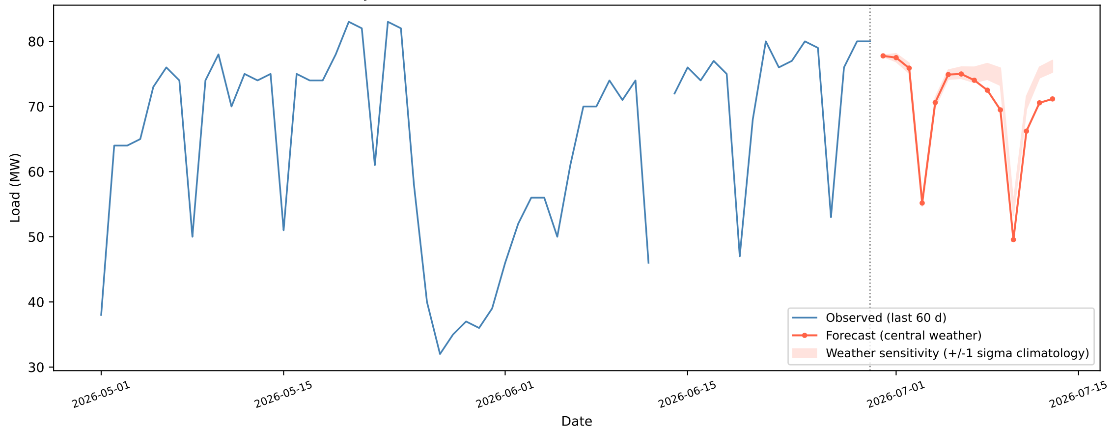
Narinda - 14-day recursive forecast (CNN+BiLSTM+BiGRU), weather mode = forecast
