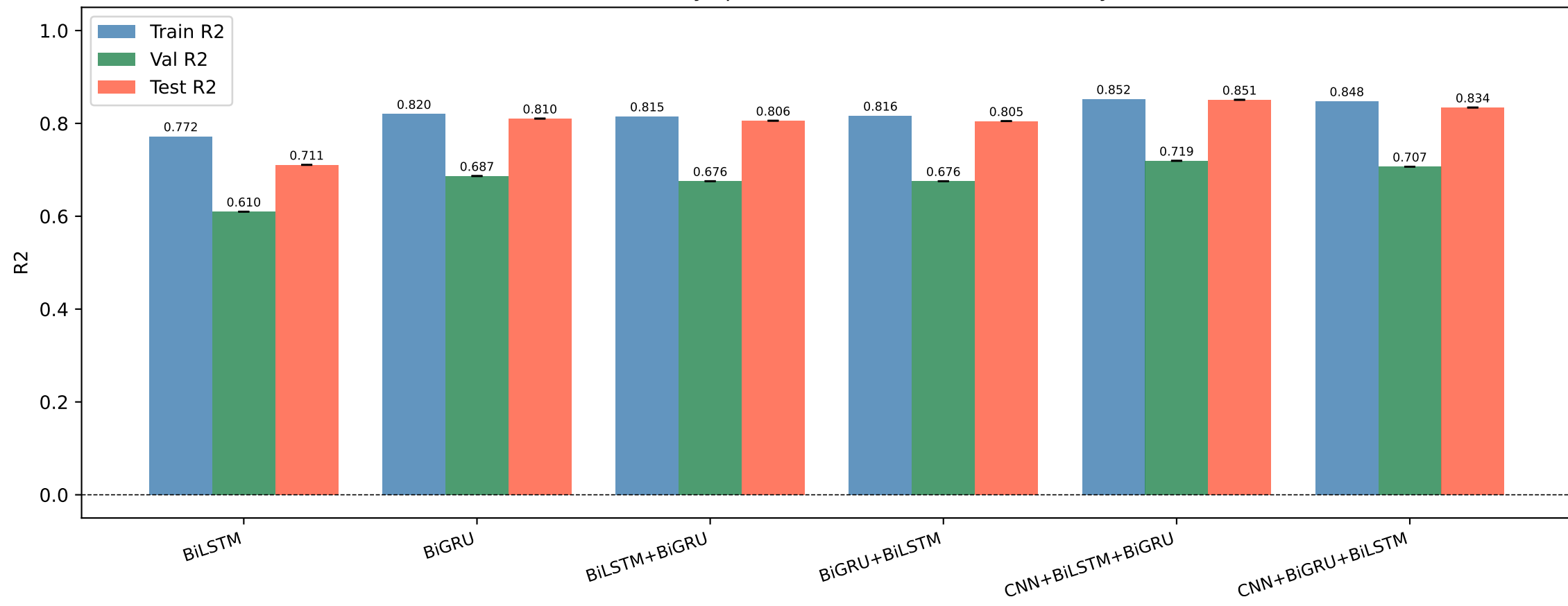
Narinda - R2 by split (model selection uses VAL only)
