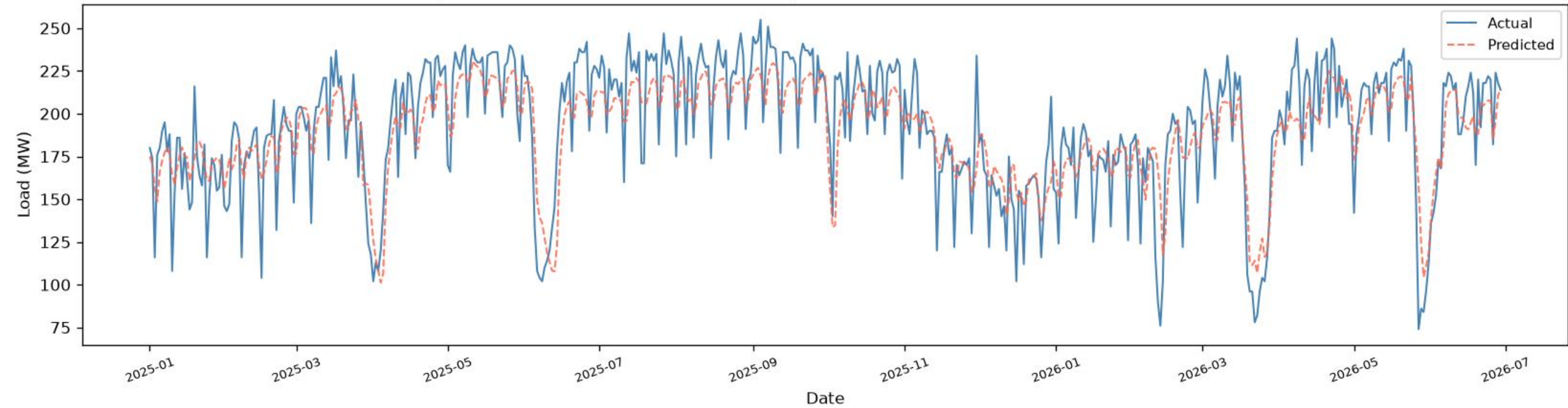
Savar | BiGRU+BiLSTM - TEST ( \geq 2025 ), one-day-ahead ( R^2=0.6937 , RMSE=21.26 , MAE=16.83 , n=533 )
