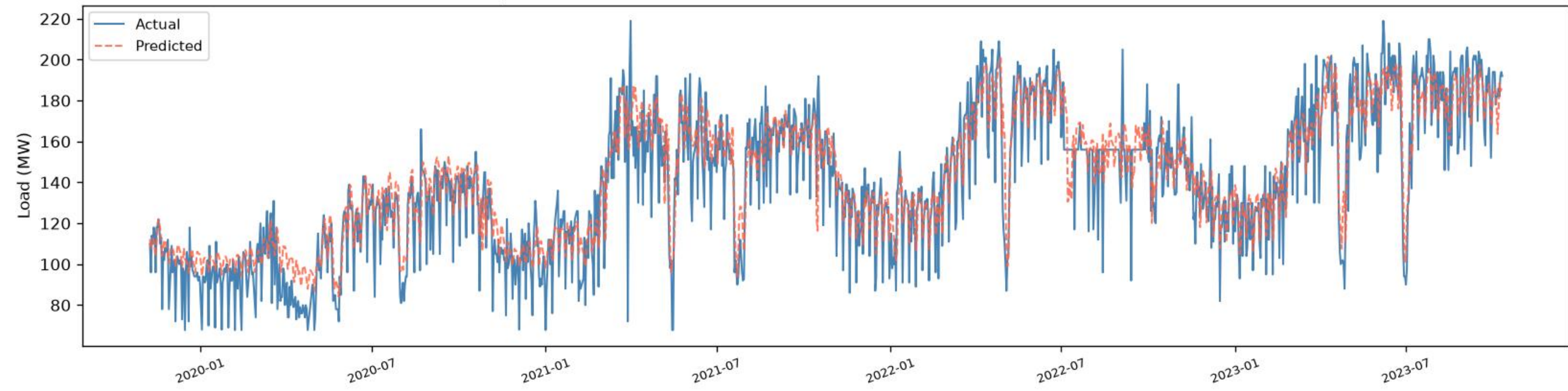
Savar | BiGRU+BiLSTM - TRAIN (fit block) ( R^2=0.8157 , RMSE=14.85, MAE=11.27, n=1386 )
