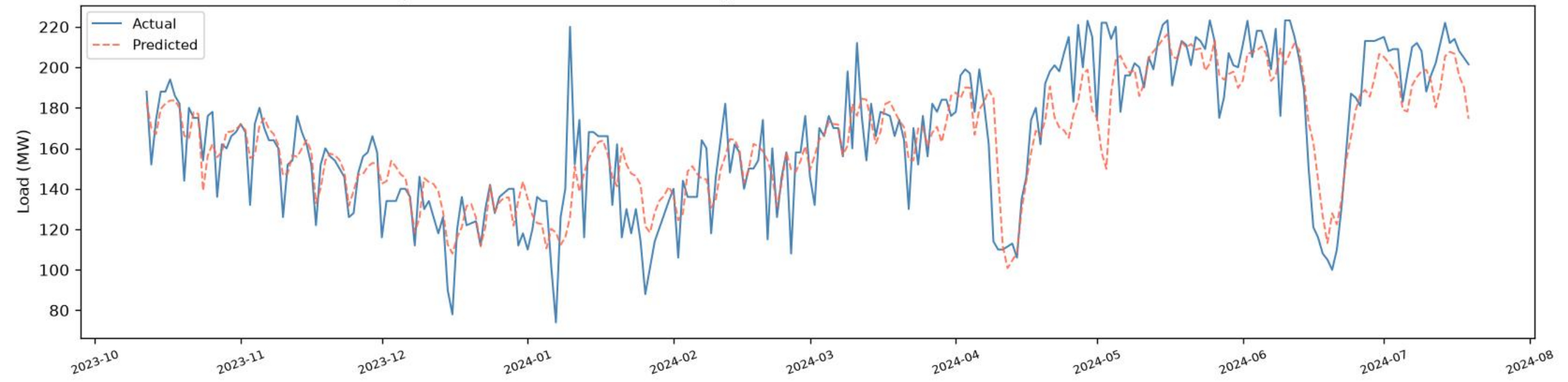
Savar | BiGRU+BiLSTM - VALIDATION (chronological, before test) ( R^2=0.7177 , RMSE=18.38, MAE=13.30, n=272)
