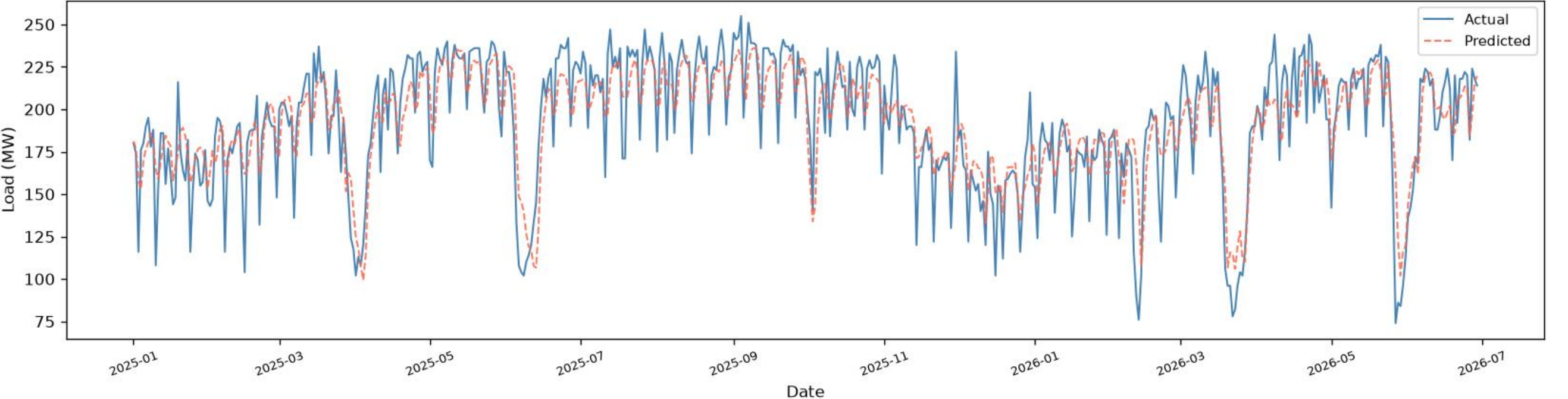
Savar | BiGRU - TEST ( \geq 2025 ), one-day-ahead (R2=0.7262, RMSE=20.10, MAE=15.43, n=533)
