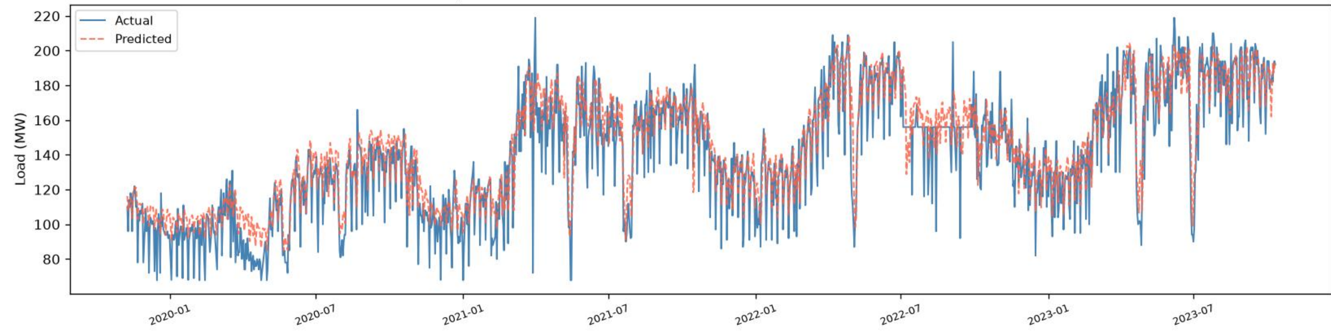
Savar | BiGRU - TRAIN (fit block) ( R^2=0.8147 , RMSE=14.89, MAE=11.26, n=1386 )
