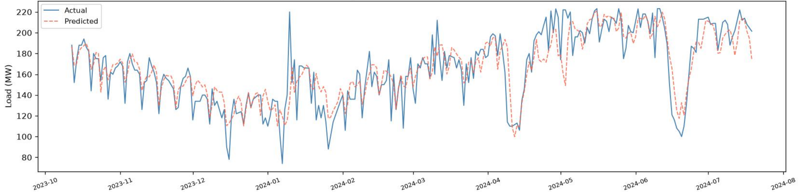
Savar | BiGRU - VALIDATION (chronological, before test) (R2=0.7300, RMSE=17.98, MAE=12.82, n=272)
