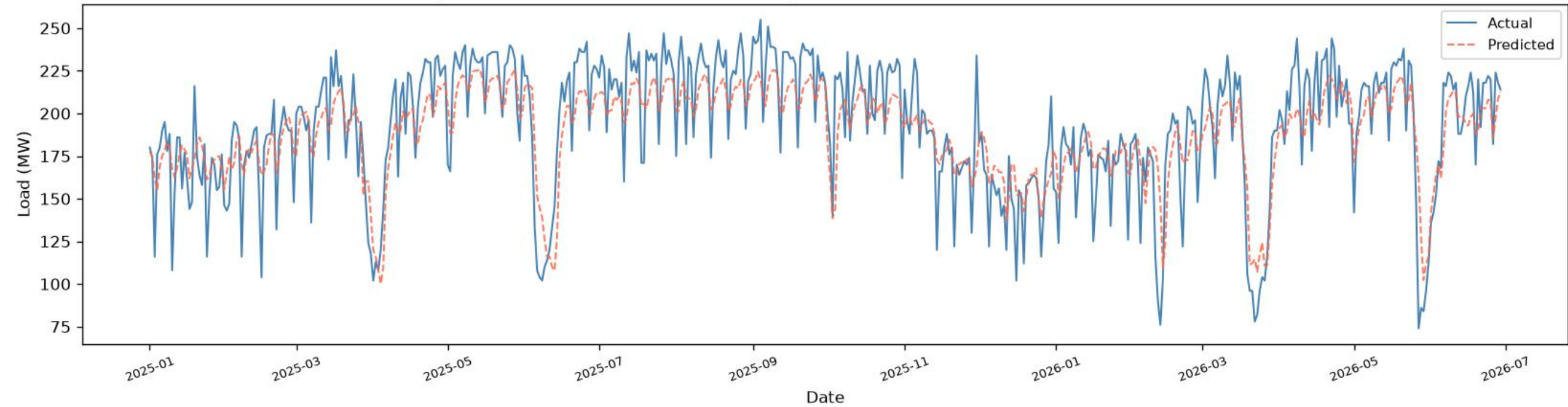
Savar | BiLSTM+BiGRU - TEST ( \geq 2025 ), one-day-ahead ( R^2=0.6856 , RMSE=21.54 , MAE=17.25 , n=533 )
