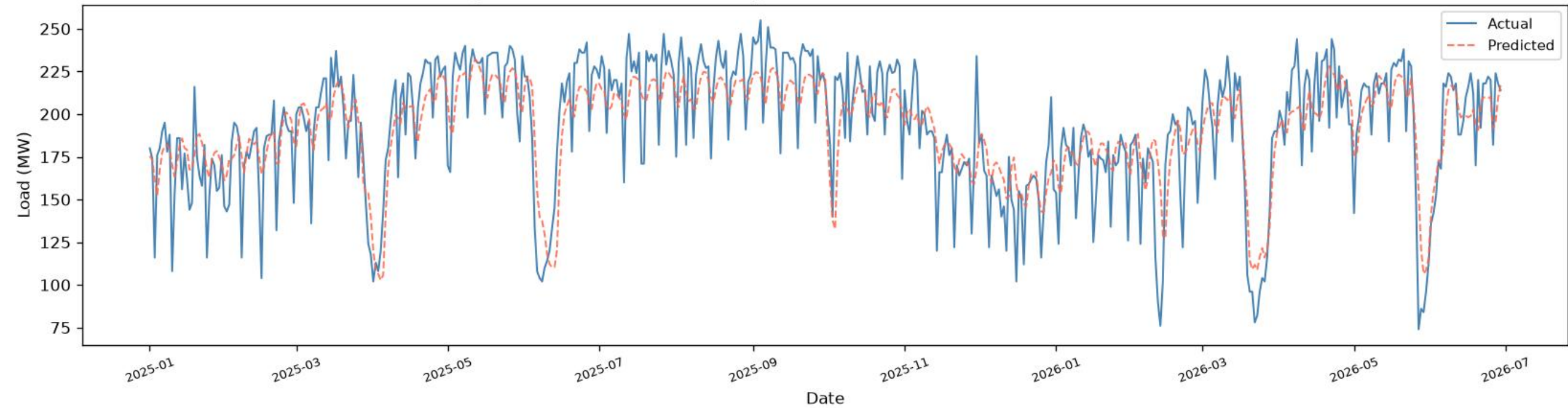
Savar | BiLSTM - TEST ( \geq 2025 ), one-day-ahead ( R^2=0.6746 , RMSE=21.91 , MAE=17.11 , n=533 )
