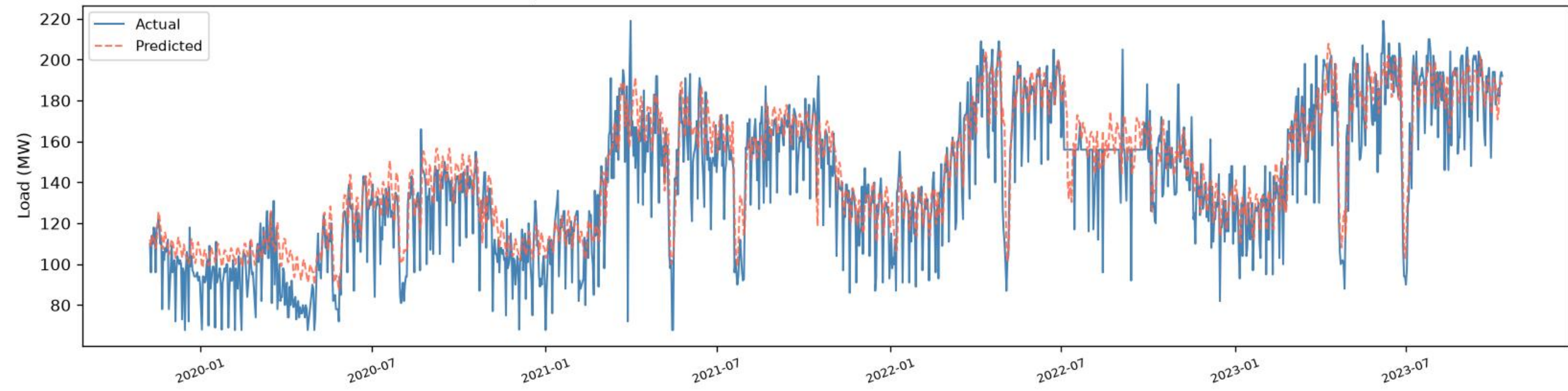
Savar | BiLSTM - TRAIN (fit block) ( R^2=0.7782 , RMSE=16.29, MAE=12.36, n=1386)
