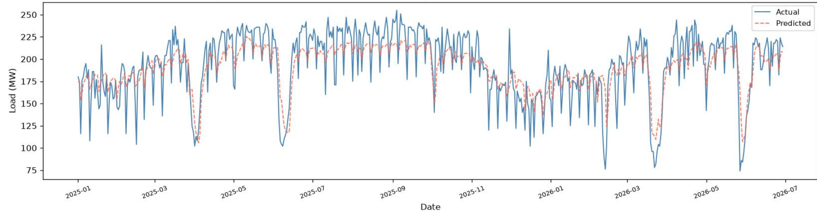
Savar | CNN+BiGRU+BiLSTM - TEST ( \geq 2025 ), one-day-ahead ( R^2=0.6781 , RMSE=21.79 , MAE=17.44 , n=533 )
