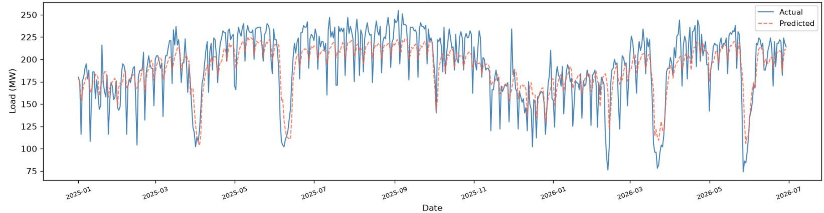
Savar | CNN+BiLSTM+BiGRU - TEST ( \geq 2025 ), one-day-ahead ( R^2=0.6930 , RMSE=21.28 , MAE=16.79 , n=533 )
