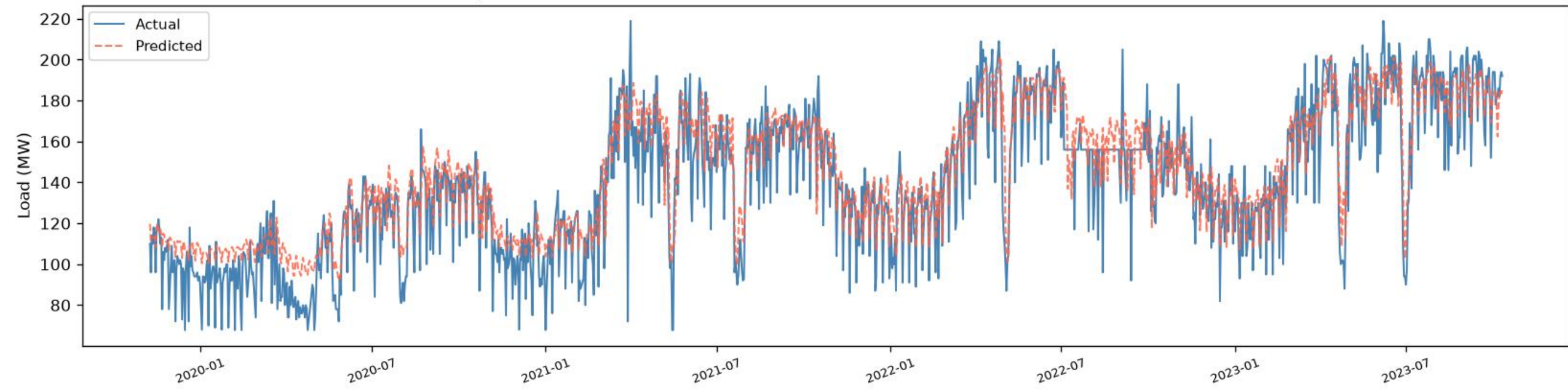
Savar | CNN+BiLSTM+BiGRU - TRAIN (fit block) (R2=0.8018, RMSE=15.40, MAE=11.71, n=1386)
