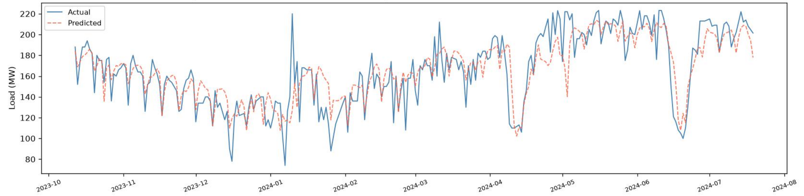
Savar | CNN+BiLSTM+BiGRU - VALIDATION (chronological, before test) ( R^2=0.7053 , RMSE=18.78, MAE=13.22, n=272)
