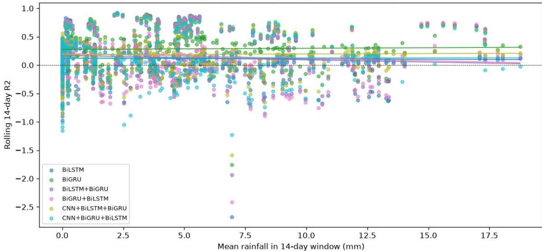
Savar - Rain vs R2 (all 6 models, test period)
