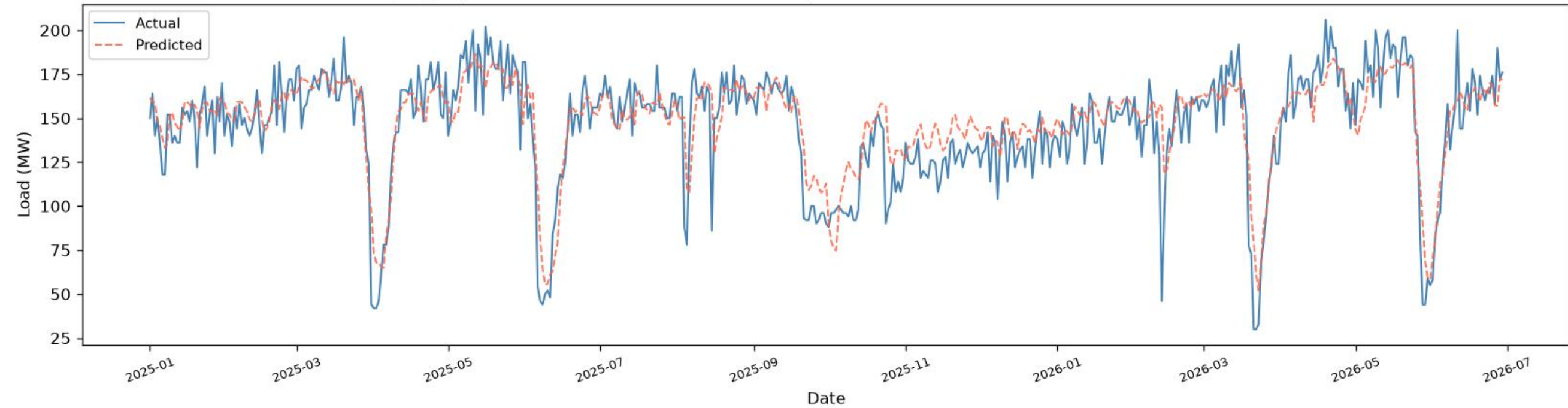
Shyampur | BiGRU+BiLSTM - TEST ( \geq 2025 ), one-day-ahead ( R^2=0.7255 , RMSE=17.18 , MAE=12.67 , n=521 )
