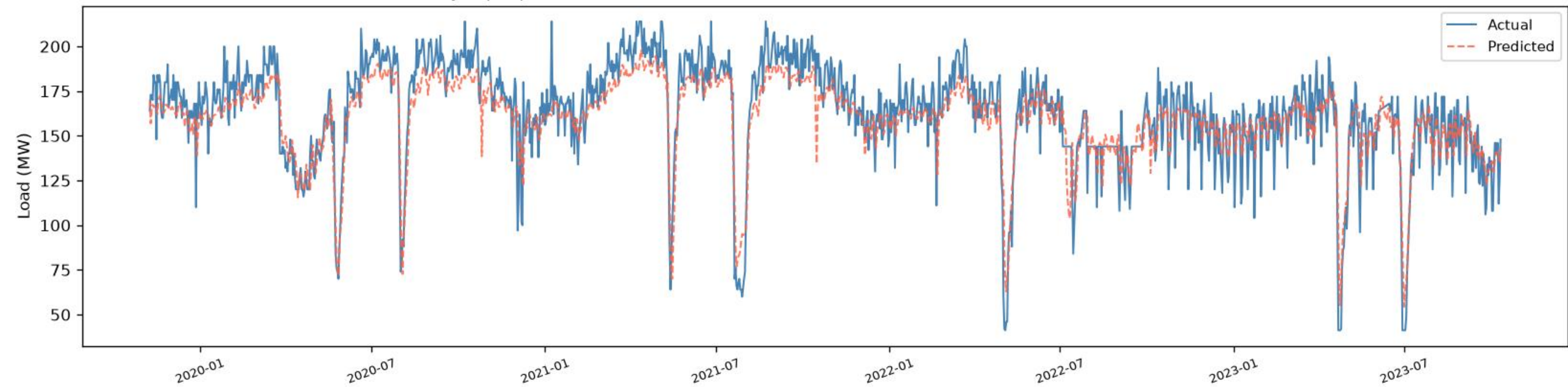
Shyampur | BiGRU+BiLSTM - TRAIN (fit block) (R2=0.7567, RMSE=14.27, MAE=11.14, n=1347)
