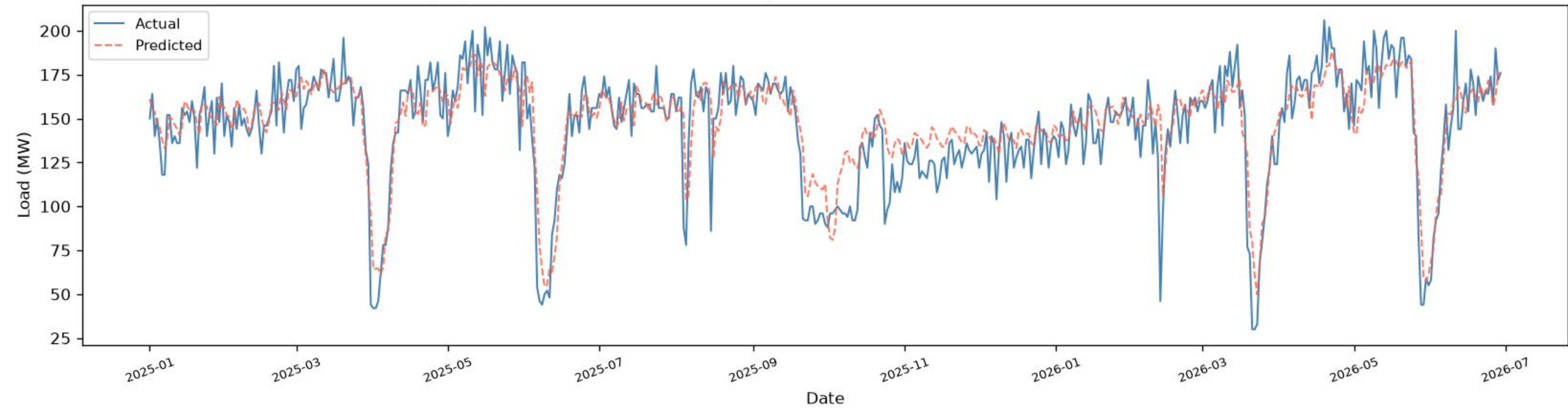
Shyampur | BiGRU - TEST ( \geq 2025 ), one-day-ahead ( R^2=0.7512 , RMSE=16.35 , MAE=11.89 , n=521 )
