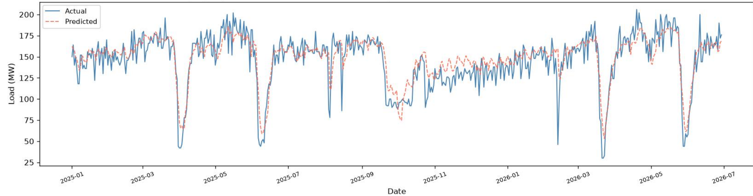
Shyampur | BiLSTM+BiGRU - TEST ( \geq 2025 ), one-day-ahead ( R^2=0.7275 , RMSE=17.11 , MAE=12.60 , n=521 )
