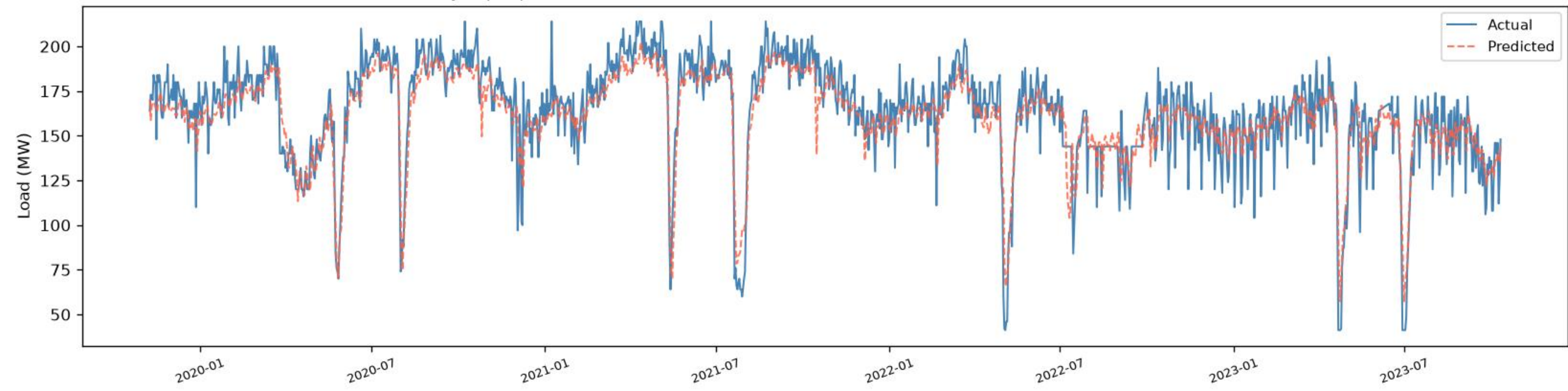
Shyampur | BiLSTM+BiGRU - TRAIN (fit block) (R2=0.7781, RMSE=13.63, MAE=10.27, n=1347)
