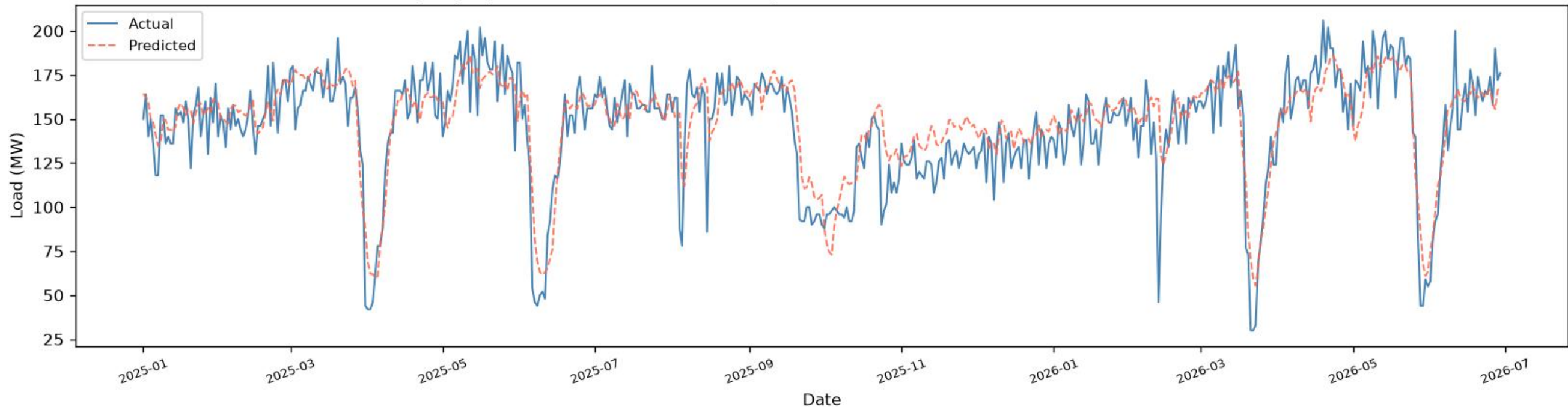
Shyampur | BiLSTM - TEST ( \geq 2025 ), one-day-ahead ( R^2=0.7212 , RMSE=17.31 , MAE=12.85 , n=521 )
