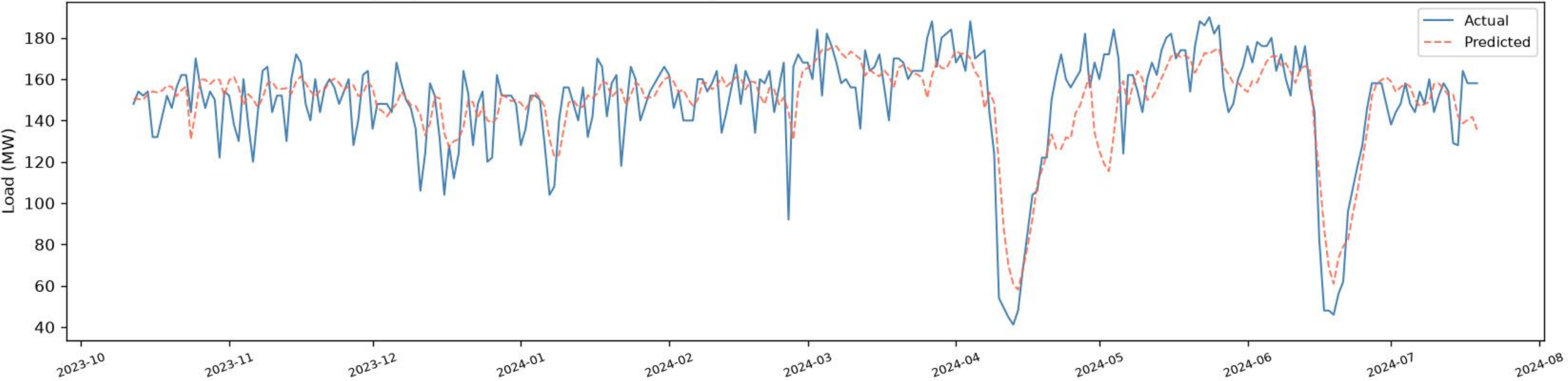
Shyampur | BiLSTM - VALIDATION (chronological, before test) (R2=0.5948, RMSE=16.64, MAE=12.64, n=269)
