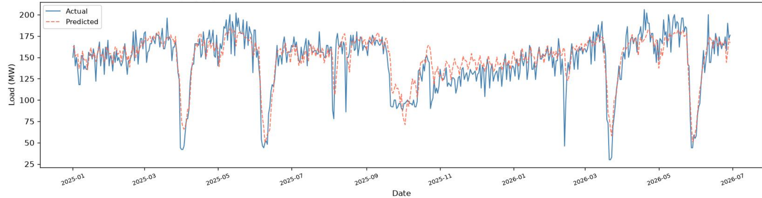
Shyampur | CNN+BiGRU+BiLSTM - TEST ( \geq 2025 ), one-day-ahead ( R^2=0.7475 , RMSE=16.47 , MAE=12.05 , n=521 )
