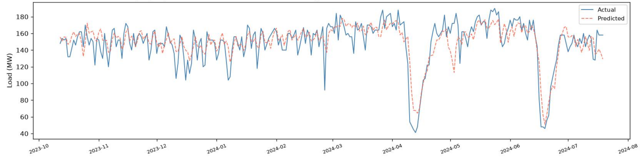
Shyampur | CNN+BiGRU+BiLSTM - VALIDATION (chronological, before test) ( R^2=0.6715 , RMSE=14.98 , MAE=11.12 , n=269 )
