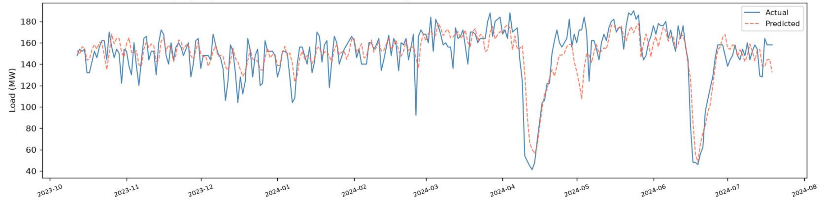
Shyampur | CNN+BiLSTM+BiGRU - VALIDATION (chronological, before test) ( R^2=0.6599 , RMSE=15.25 , MAE=11.10 , n=269 )
