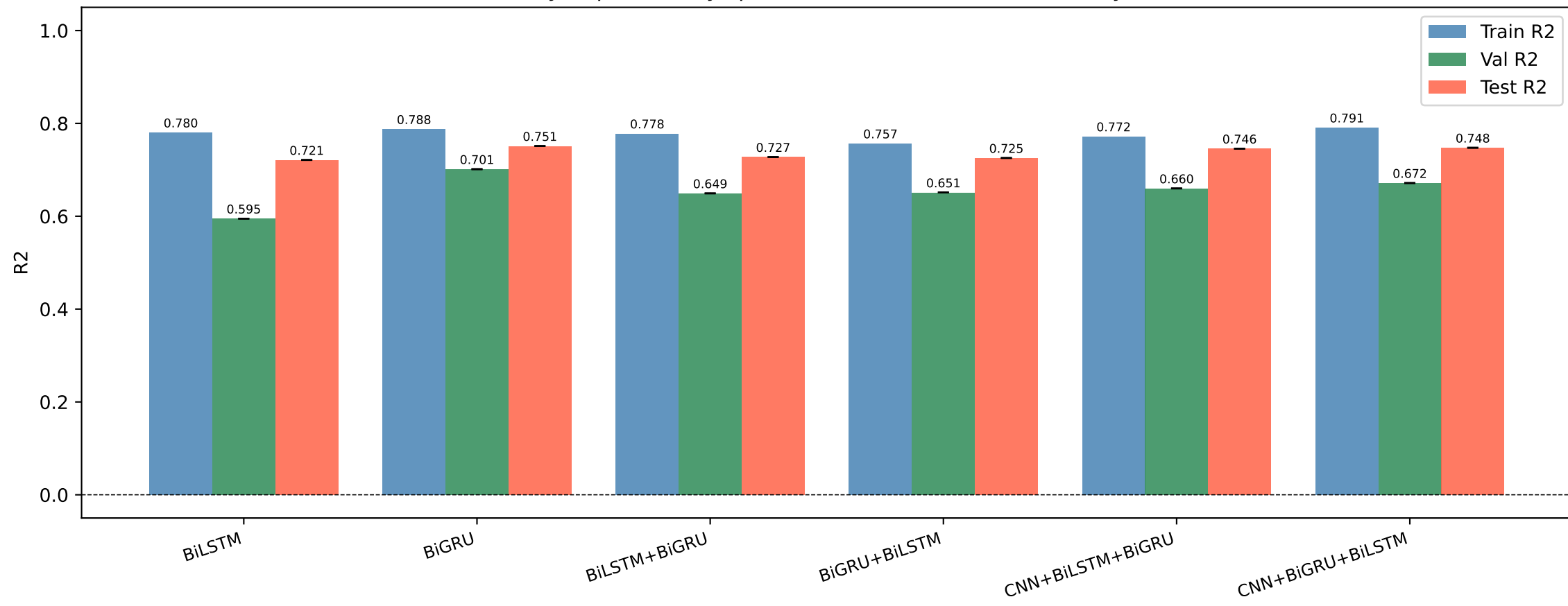
Shyampur - R2 by split (model selection uses VAL only)
