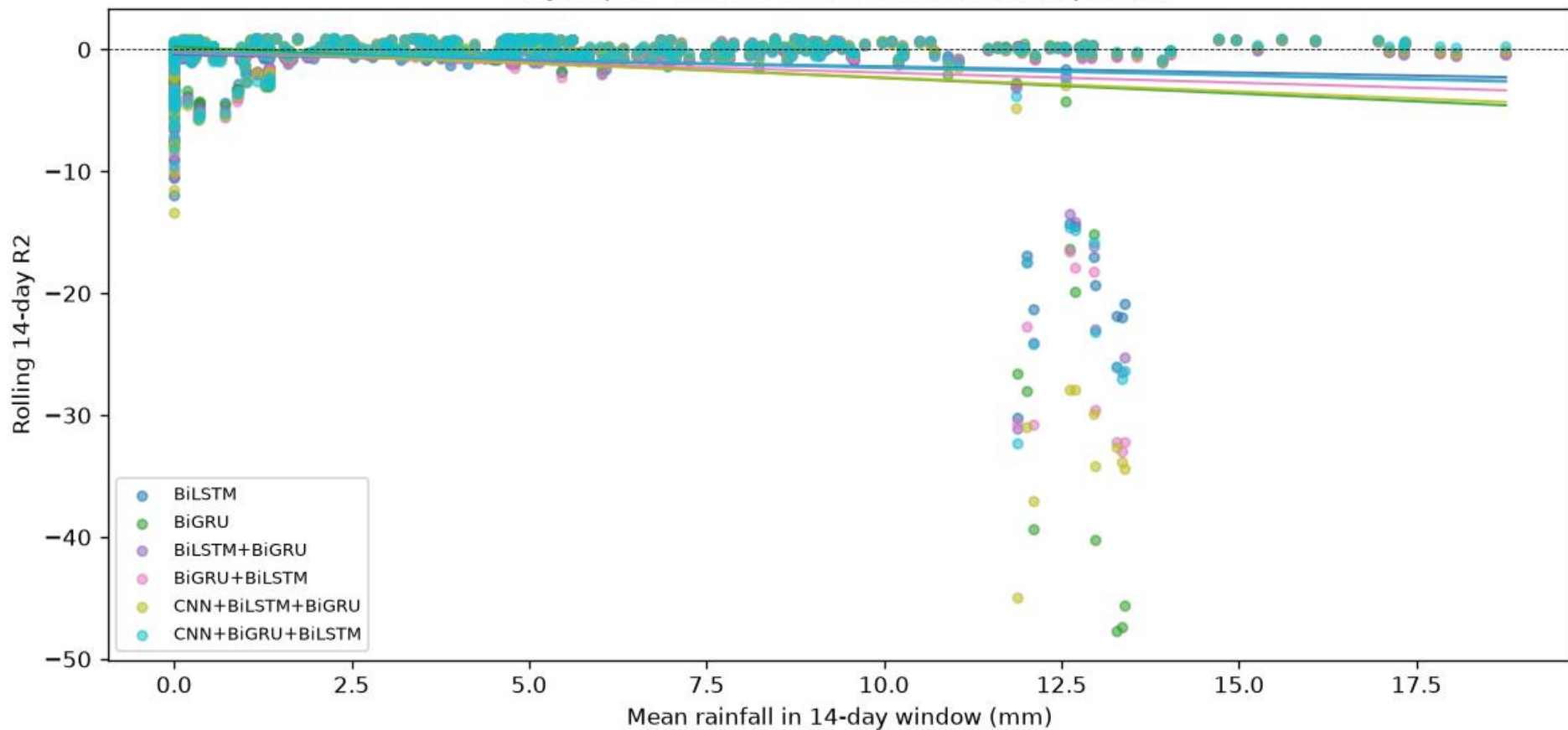
Shyampur - Rain vs R2 (all 6 models, test period)
