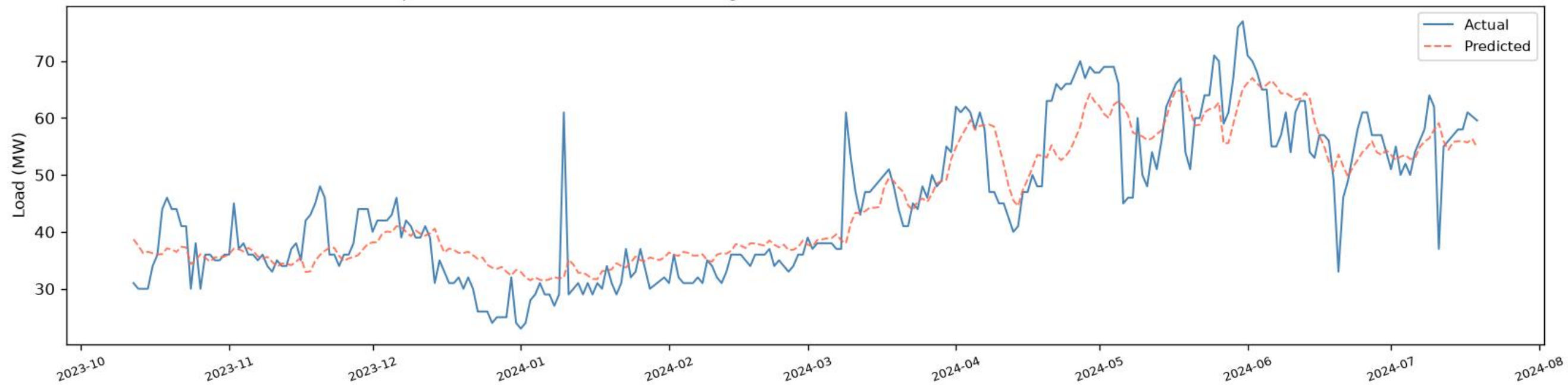
Ullon | BiGRU+BiLSTM - VALIDATION (chronological, before test) (R2=0.7762, RMSE=6.13, MAE=4.49, n=272)
