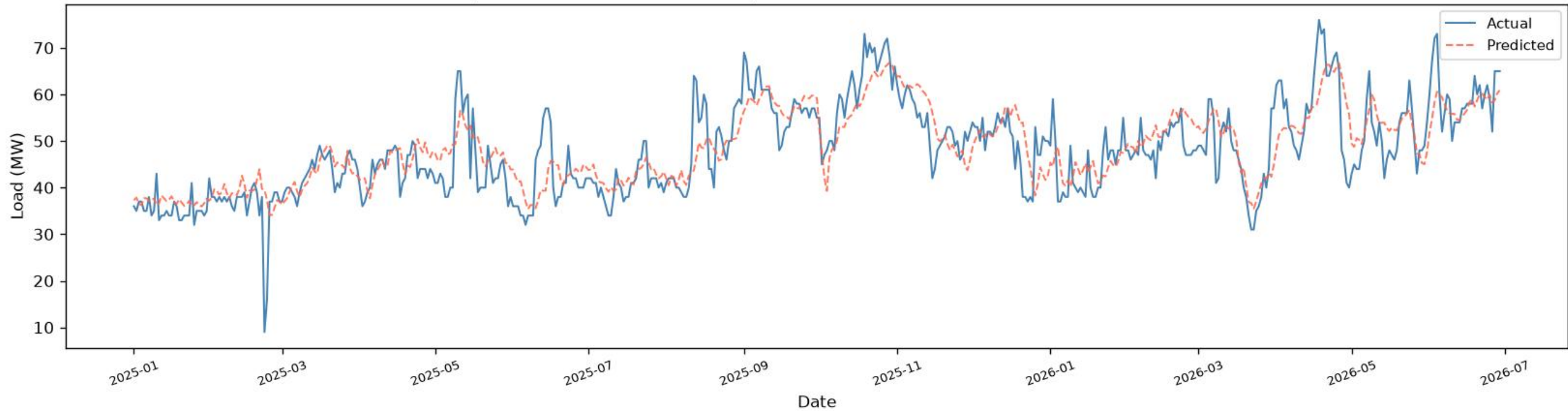
Ullon | BiGRU - TEST ( \geq 2025 ), one-day-ahead ( R^2=0.6508 , RMSE=5.75 , MAE=4.29 , n=536 )
