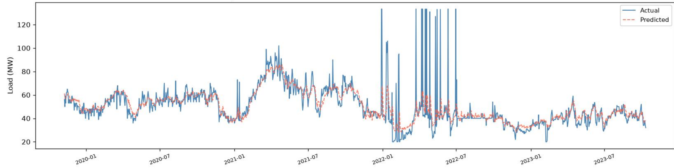
Ullon | BiGRU - TRAIN (fit block) ( R^2=0.5714 , RMSE=10.64, MAE=5.05, n=1385)
