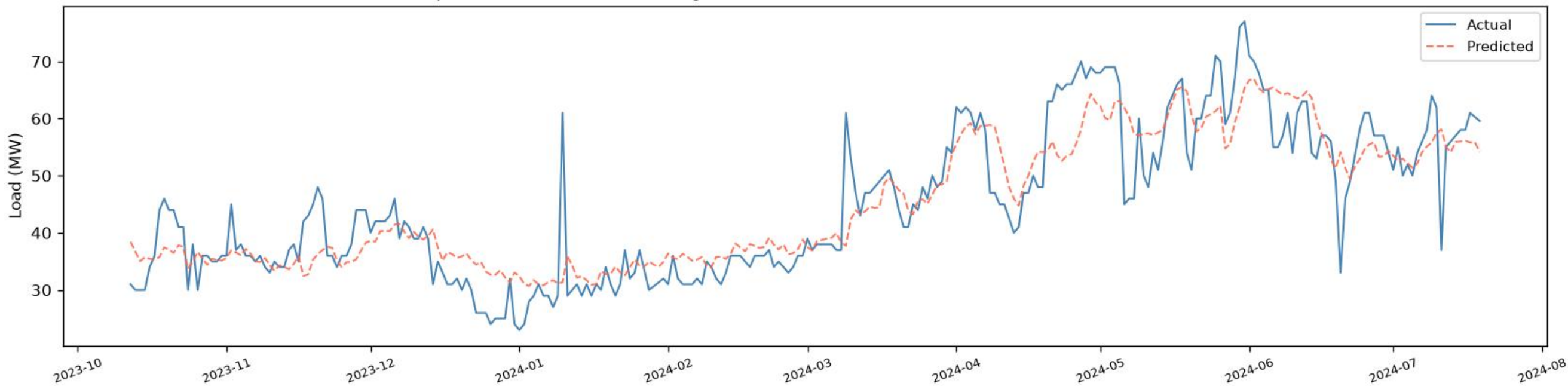
Ullon | BiGRU - VALIDATION (chronological, before test) (R2=0.7816, RMSE=6.06, MAE=4.41, n=272)
