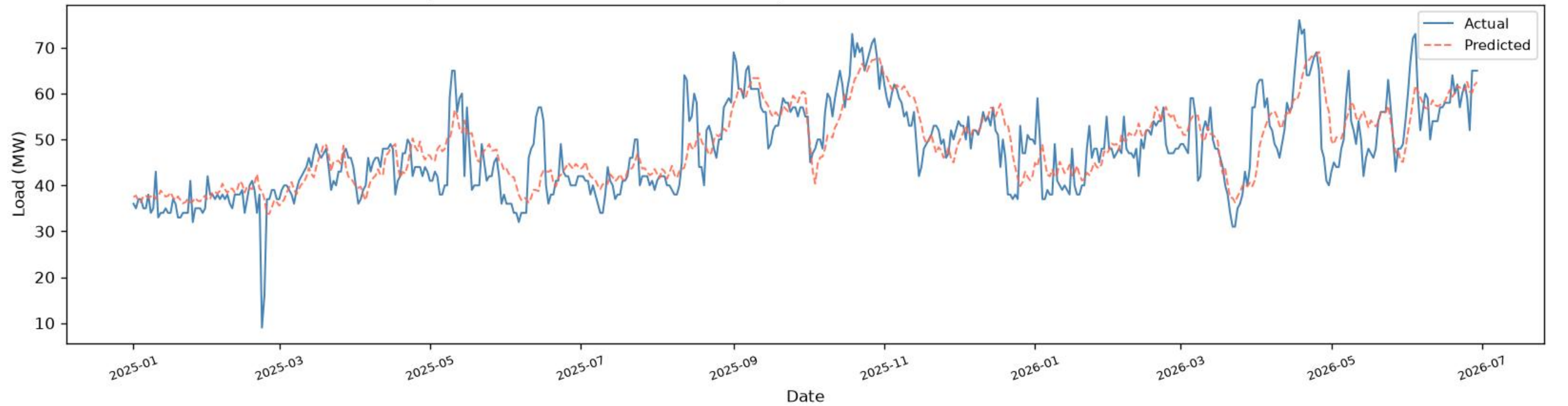
Ullon | BiLSTM+BiGRU - TEST ( \geq 2025 ), one-day-ahead ( R^2=0.6399 , RMSE=5.84 , MAE=4.41 , n=536 )
