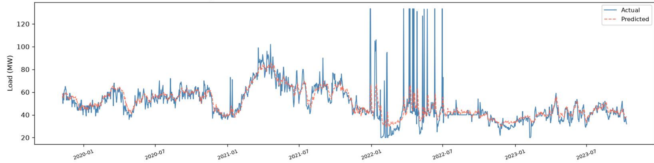
Ullon | BiLSTM+BiGRU - TRAIN (fit block) ( R^2=0.5648 , RMSE=10.73 , MAE=5.11 , n=1385 )
