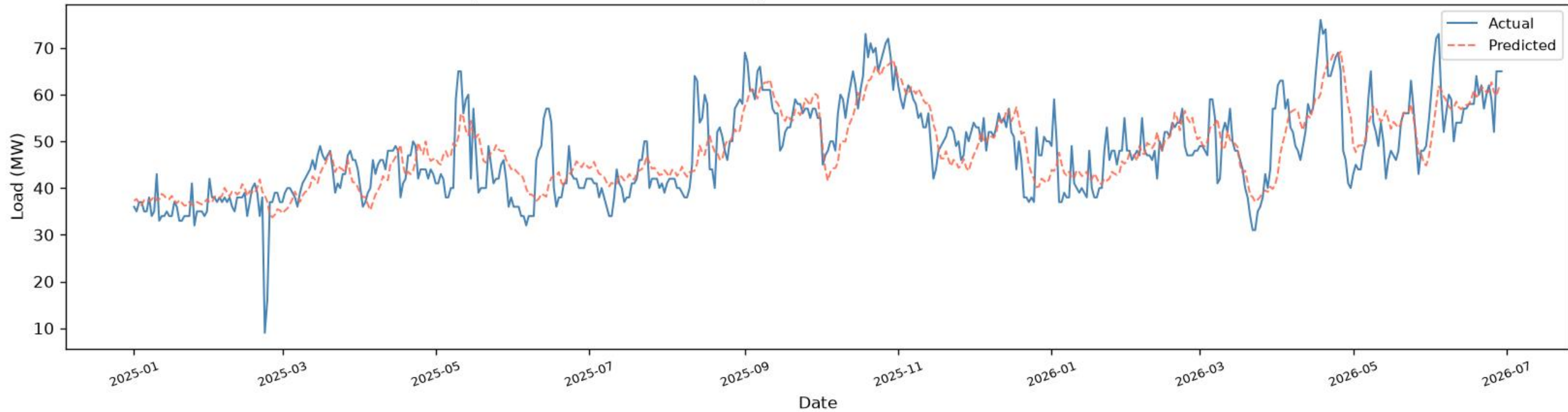
Ullon | BiLSTM - TEST ( \geq 2025 ), one-day-ahead ( R^2=0.6227 , RMSE=5.98 , MAE=4.56 , n=536 )
